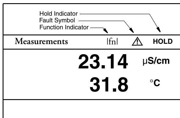
Figure 4. Typical Dual Measurement Display
