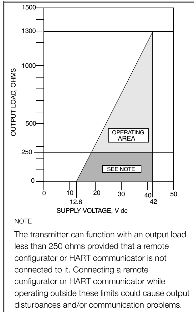
Figure 5. HART 4 to 20 mA Output, Supply Voltage vs. Output Load
